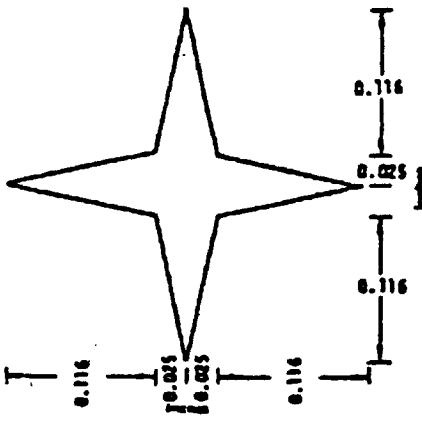
S22 STANDARD WAYPOINT SYMBOL
